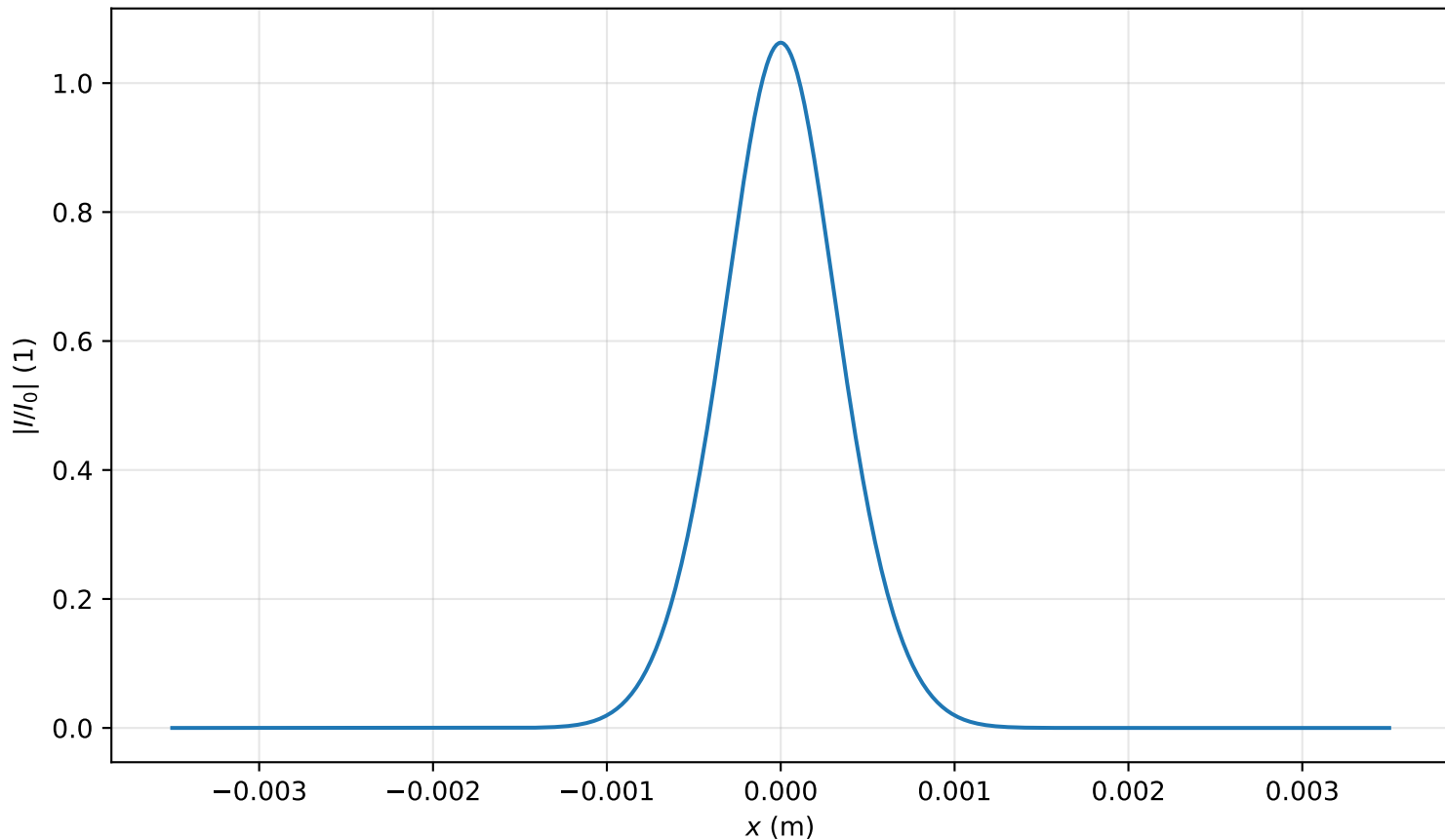
Intensity profile I(x, y = 0, z = 0.478m)/I_0 , P_{in}=0.6P_{cr} , artificial time
